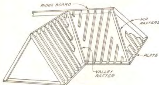
HIP AND VALLEY RAFTERS.
